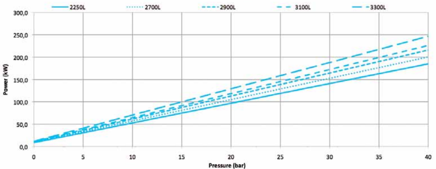
GR150 - Power @ 1450 RPM - 46 cSt
