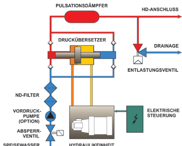
System diagram for high pressure pump ECOTRON®
