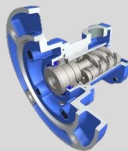
SMT8B – compact cooling and filtration
