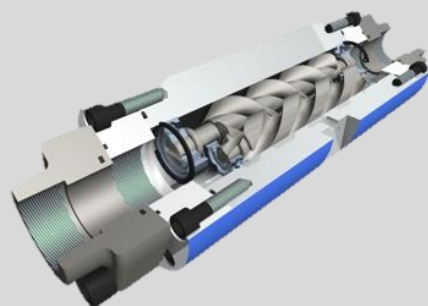
FL – high pressure flow measurement
