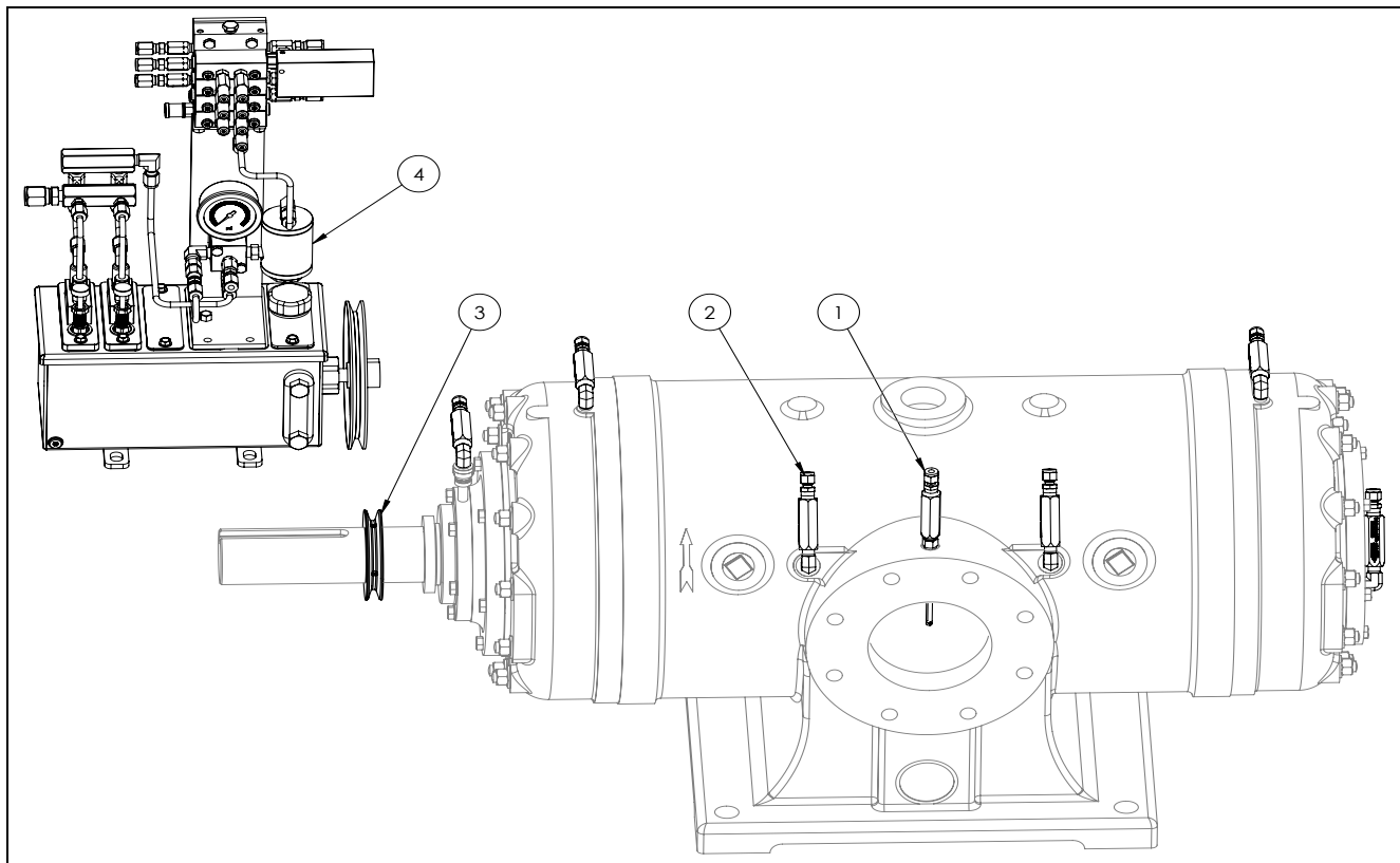
FIGURE 1 - Example of lubrication accessory installation. Refer to the model specific General Arrangement drawings available on the Ro-Flo Compressors website at www.roflocompressors.com , for specific installation locations.
