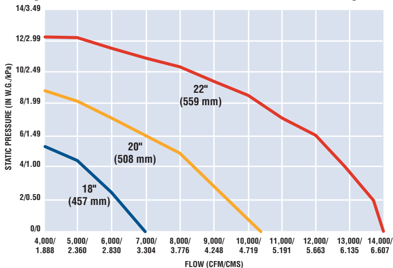
Shogun Modular Fan Curves, 3125 RPM, 0.075 lb/ft 3 [1.201 kg/m 3 ]
