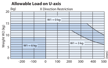
Distance between Center of U-axis Rotation and Load Gravity
